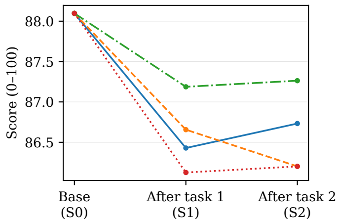
Math \rightarrow IFEval: GSM8K exact match
