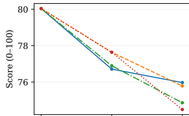
Math \rightarrow IFEval: IFEval strict accuracy
