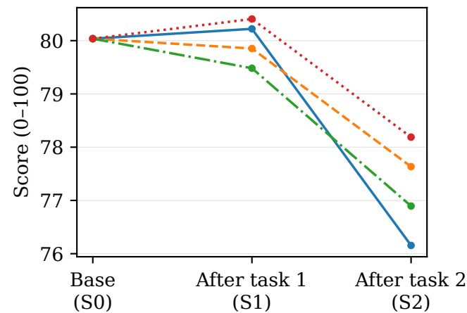
Math \rightarrow IFEval: IFEval strict accuracy
