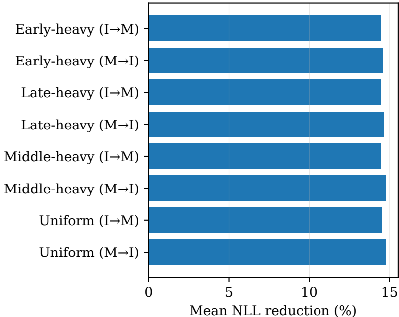
Training-derived calibration
