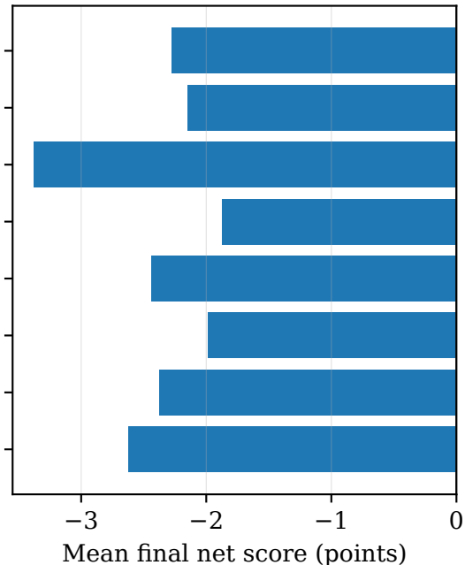
Held-out benchmarks
