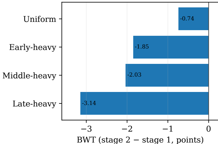
IFEval learned first
