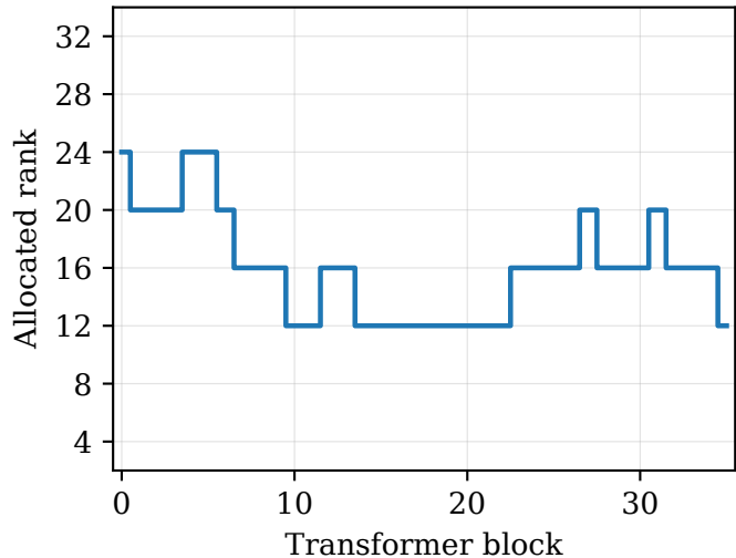
Allocated rank after the discarded pilot
