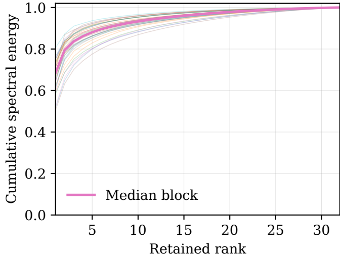
Factorized update energy
