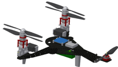
Figure 1: Coaxial tilt rotor UAV.
