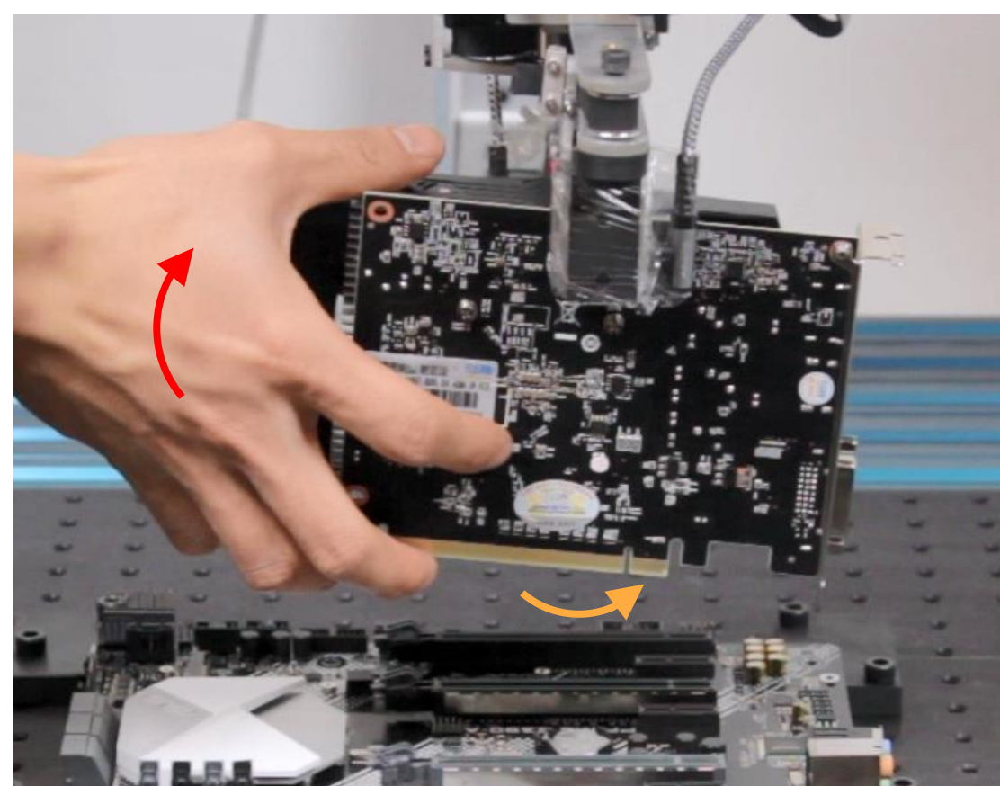
(a) Motherboard assembly under human disturbance
