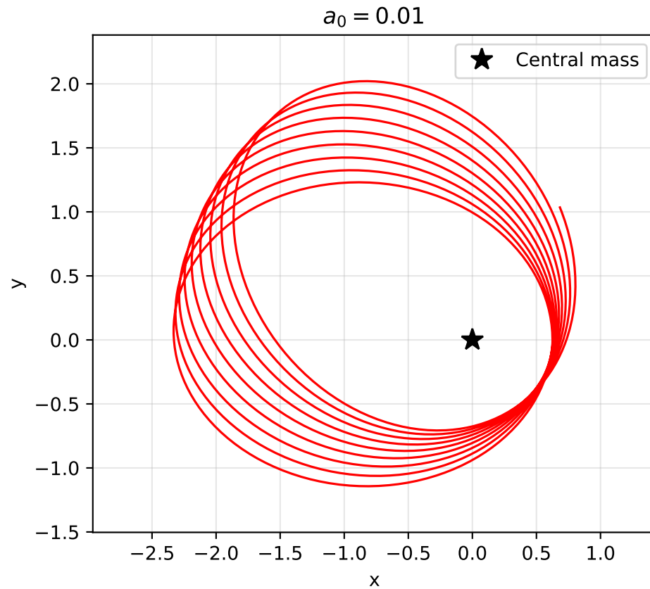
Figure 1: MOND Orbits (GM=1, h=1, e=0.6)
