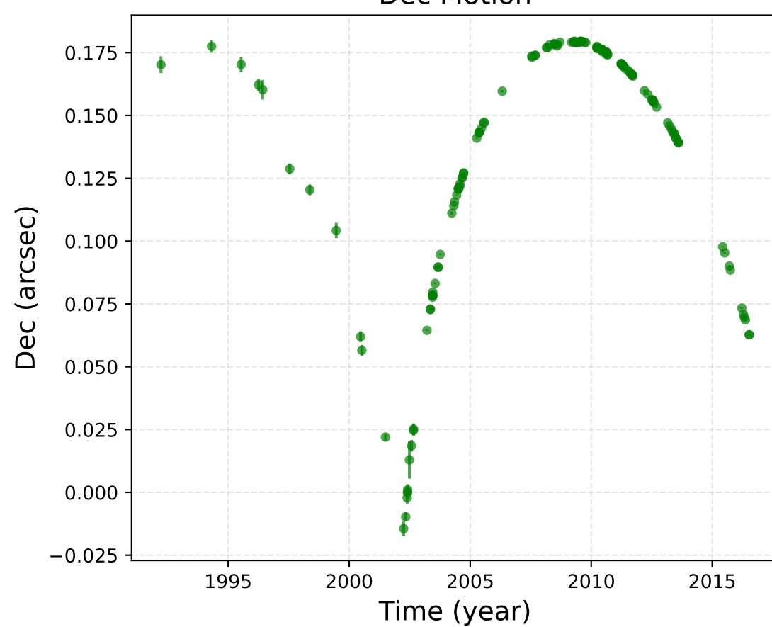
Dec Motion
