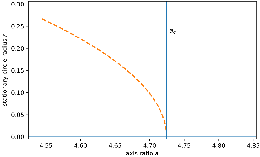
Figure 1: Certified local bifurcation picture. The dashed curve represents the leading law r_*(a)^2 = c(a_c - a) . The coefficient satisfies the certified enclosure c \in [0.3415, 0.4516] ; 0.39474123 is a non-certified reference-point estimate. The figure is schematic, not a global numerical continuation.
