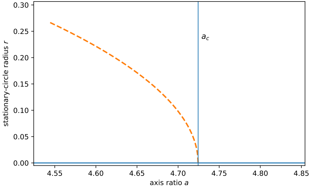
Figure 1: Certified local bifurcation picture. The dashed curve represents the leading law r_*(a)^2 = c(a_c - a) . The coefficient satisfies the certified enclosure c \in [0.3415, 0.4517] ; 0.39474123 is a non-certified reference-point estimate. The figure is schematic, not a global numerical continuation.
