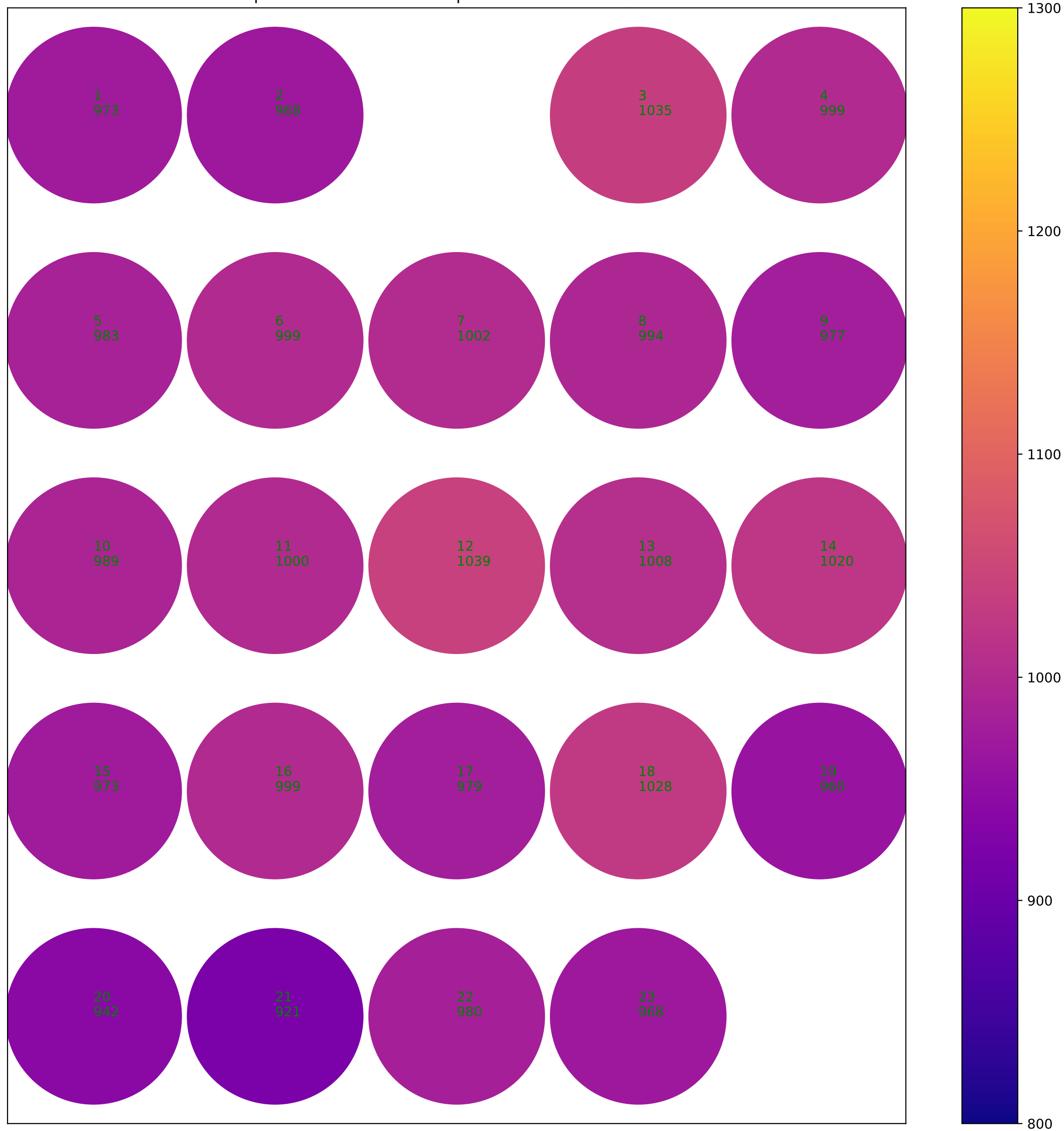
map of FR4 thickness. Each pixel is a measurement hole
