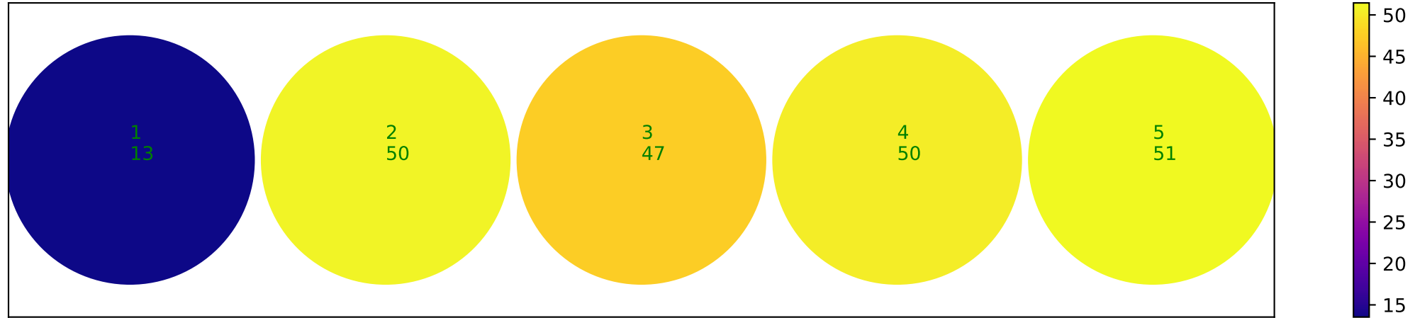
map of rim thickness. Each pixel is a measurement hole
