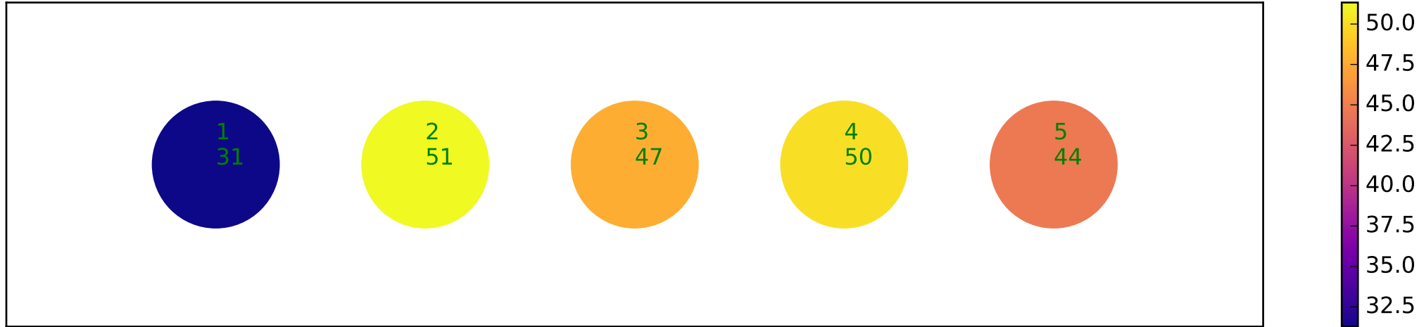
map of rim thickness. Each pixel is a measurement hole
