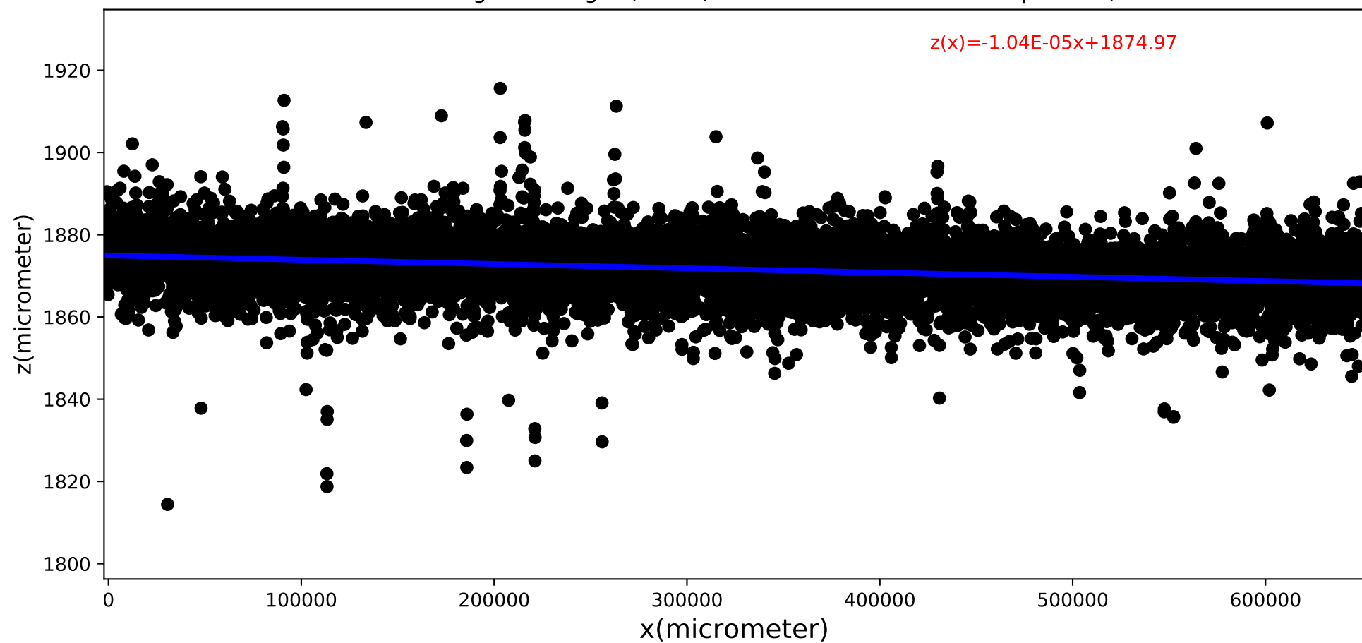
Marble Height vs length (z vs x, z histo before and after slope corr.)
