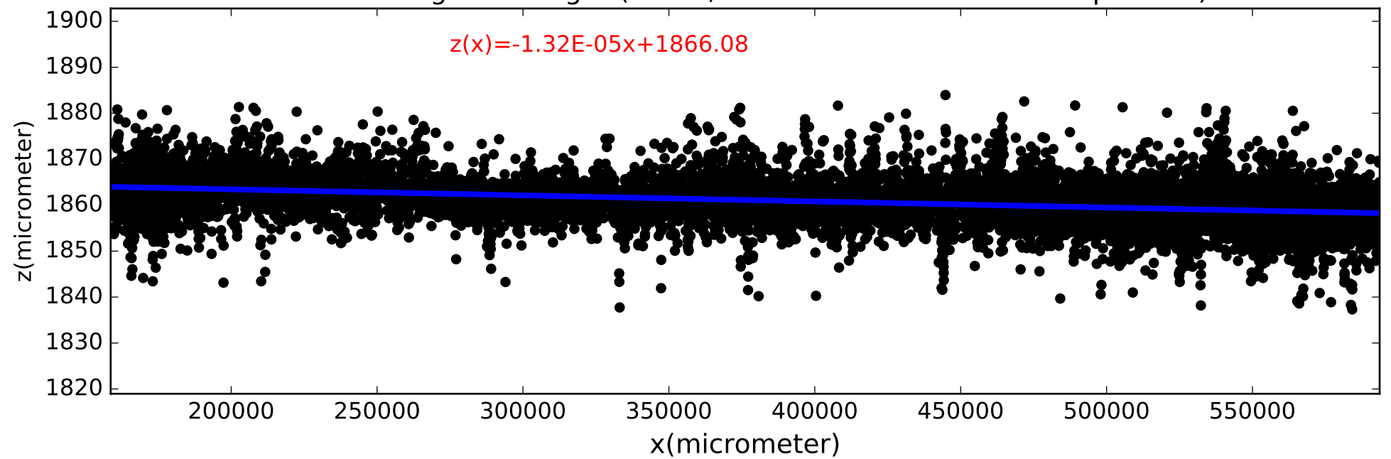
Marble Height vs length (z vs x, z histo before and after slope corr.)
