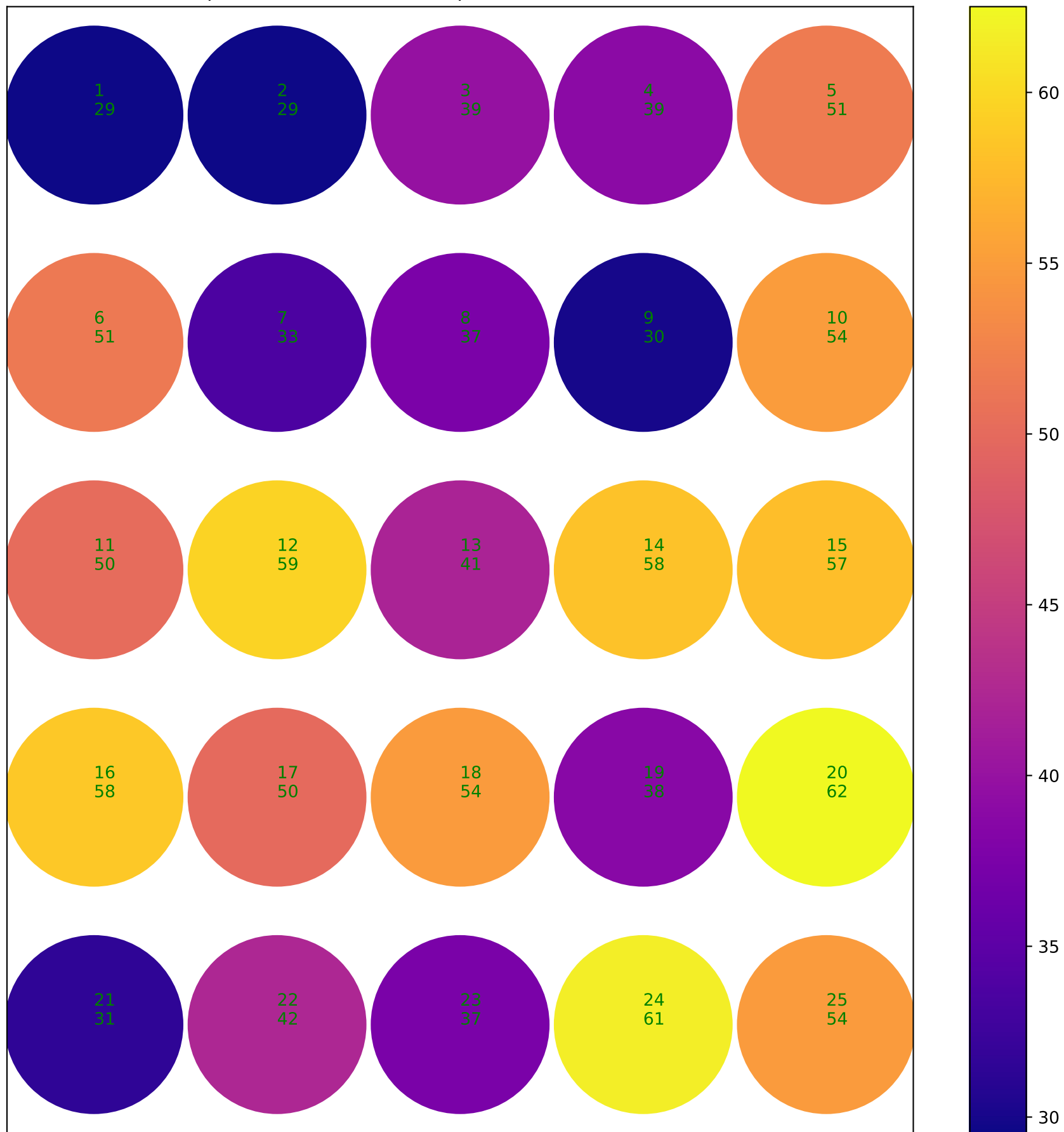
map of rim thickness. Each pixel is a measurement hole
