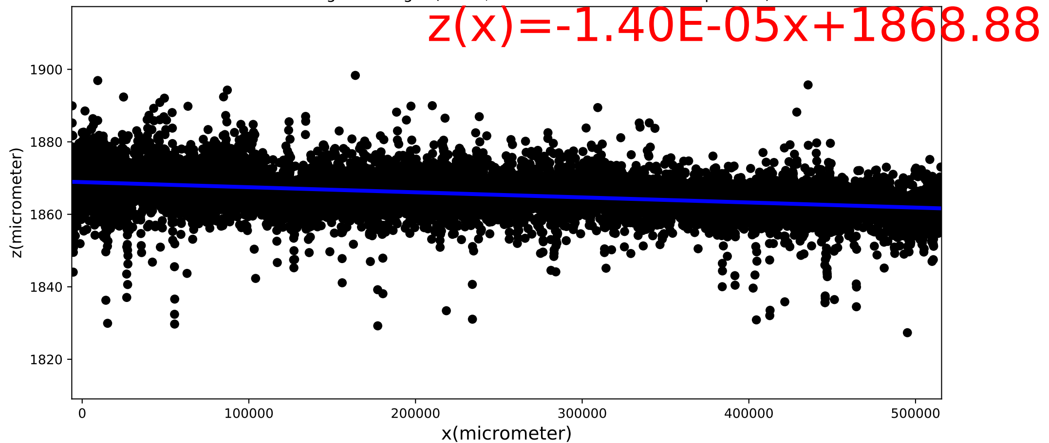
Marble Height vs length (z vs x, z histo before and after slope corr.)
