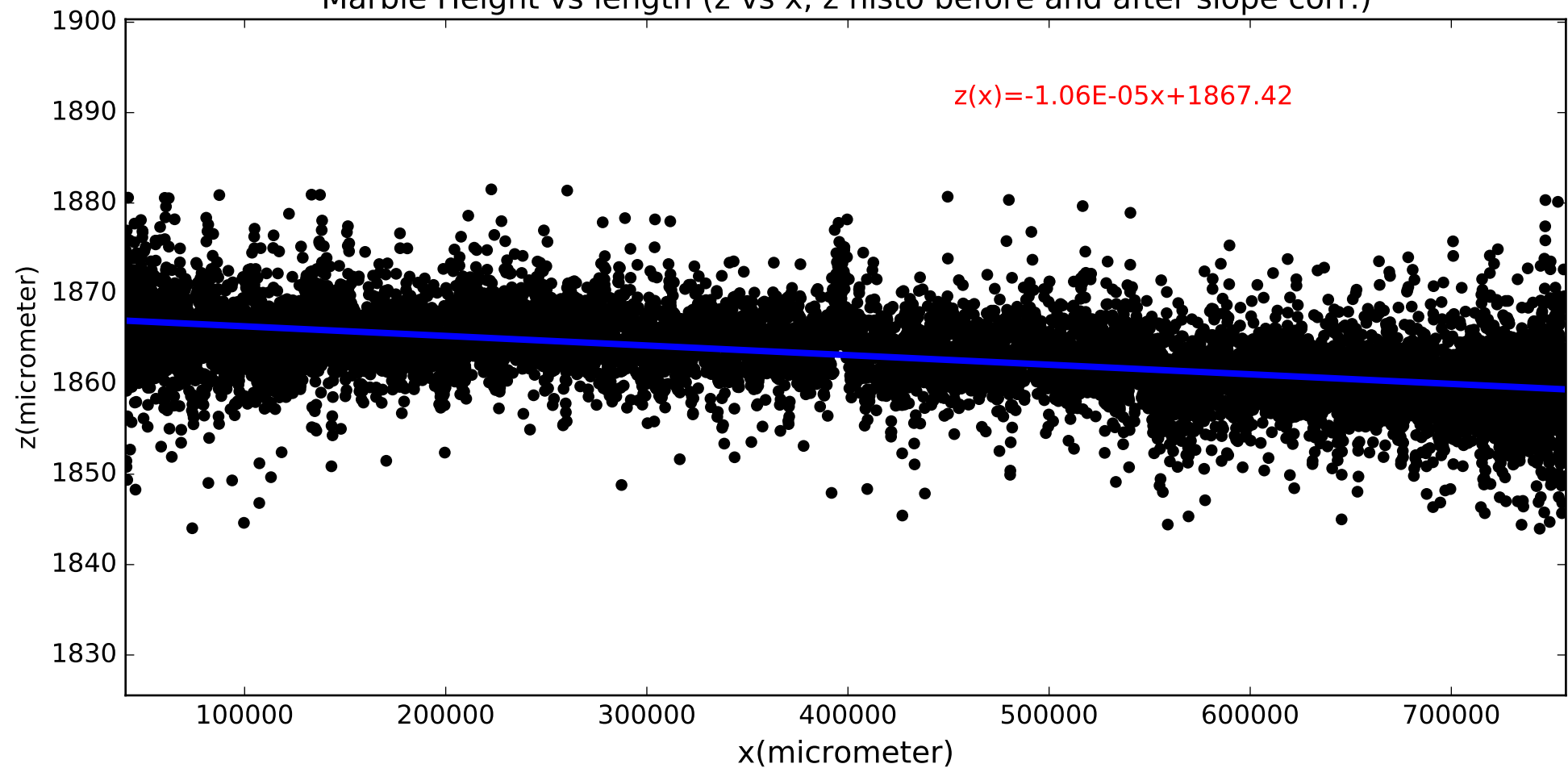
Marble Height vs length (z vs x, z histo before and after slope corr.)
