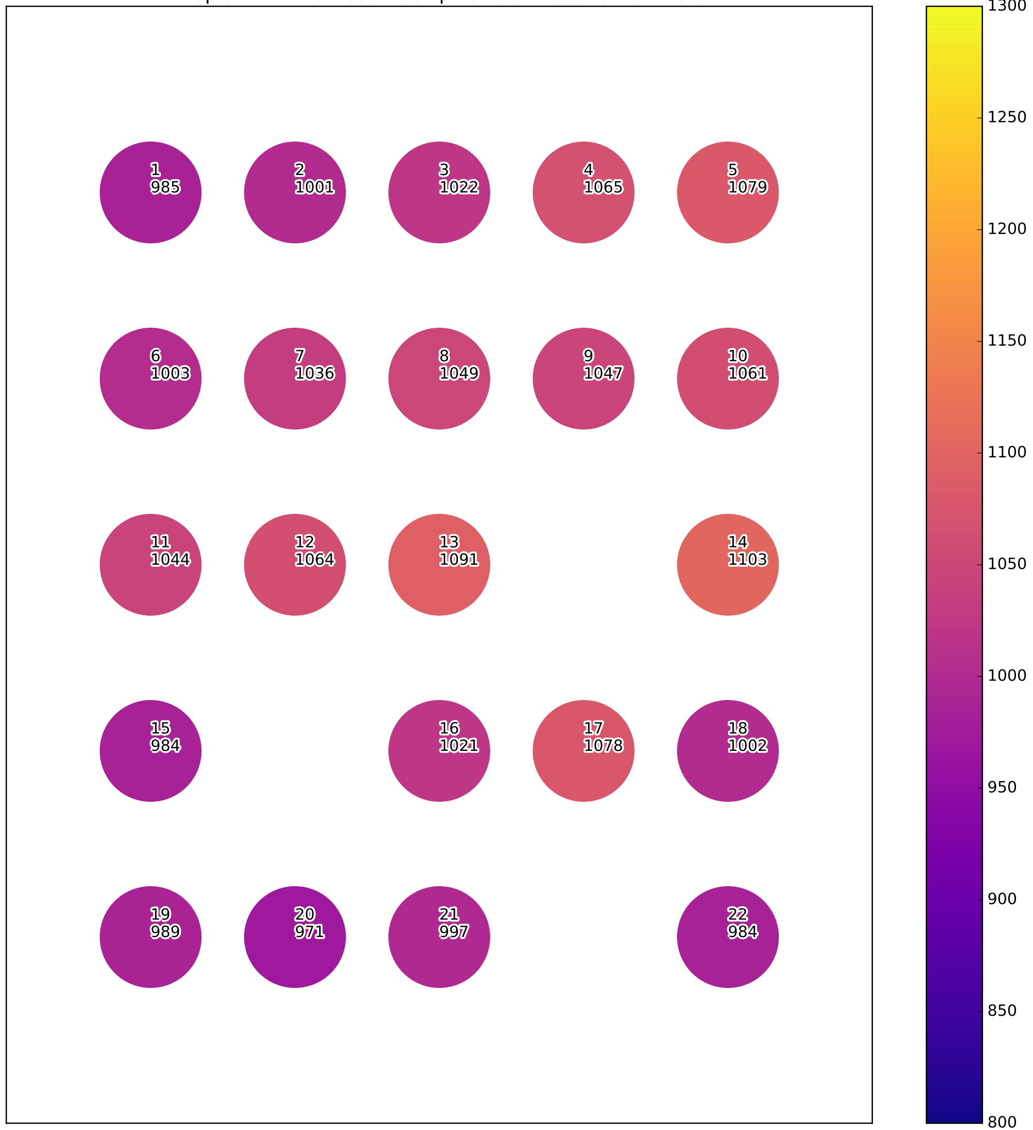
map of FR4 thickness. Each pixel is a measurement hole
