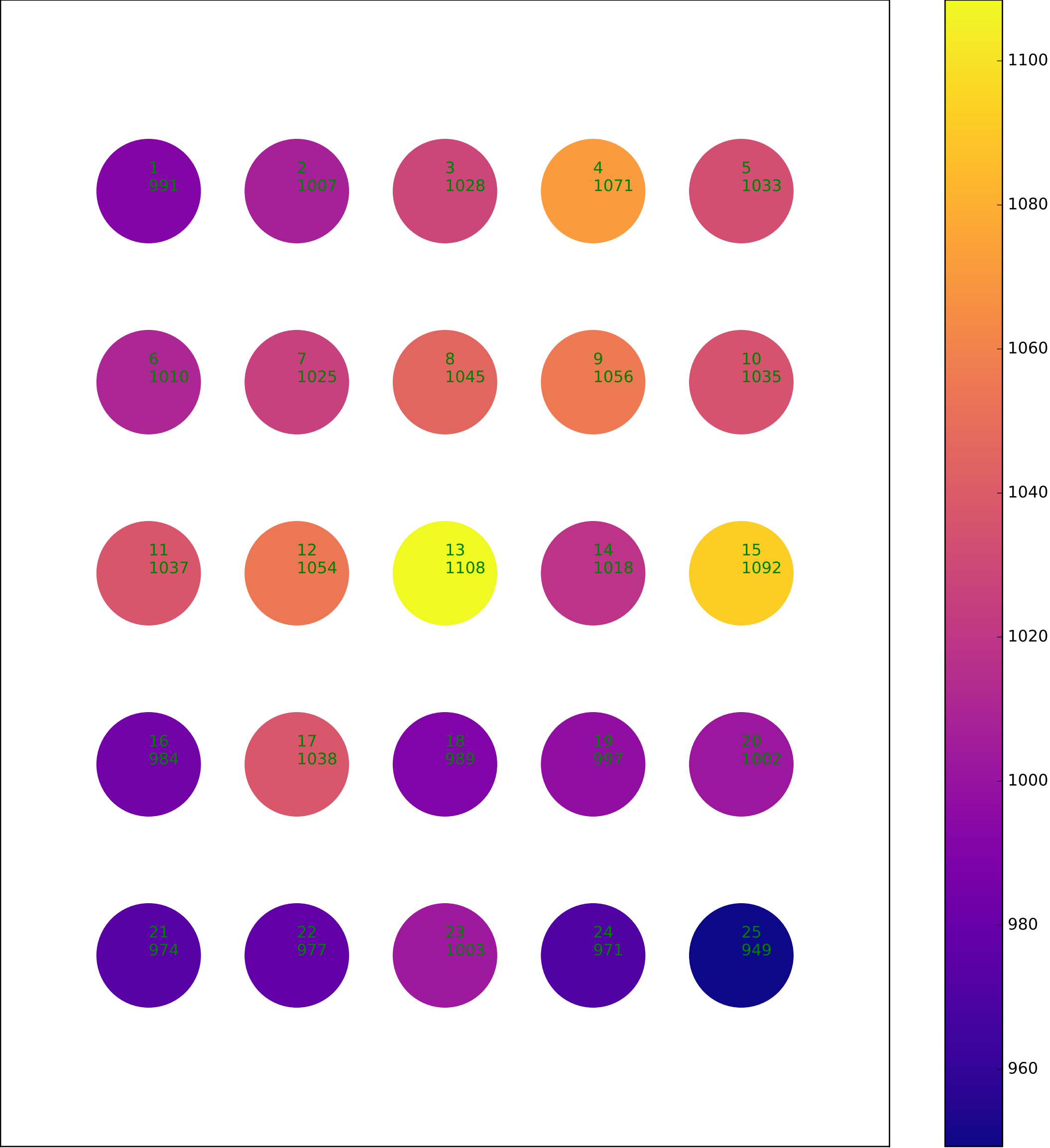
map of LEM thickness. Each pixel is a measurement hole
