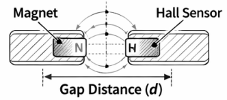
Sensing Principle (Side Cross-Section)
