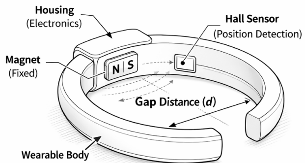
Gap Motion Range
