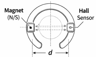
Sensing Principle (Side Cross-Section)
