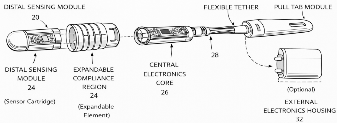
EXPLODED COMPONENT ARCHITECTURE
