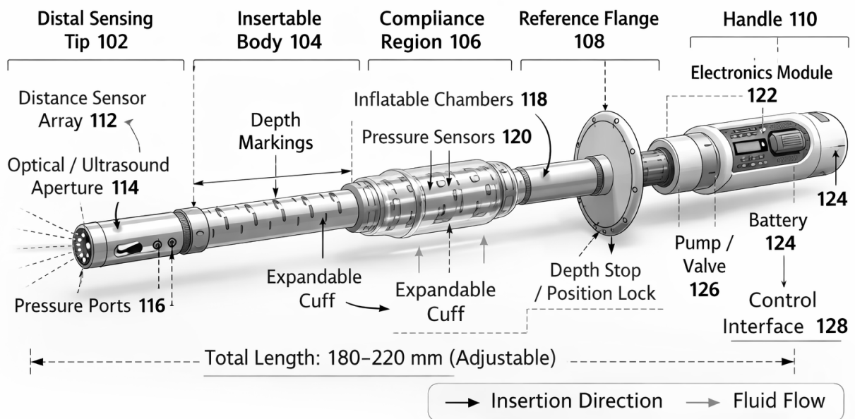
FIG. 4A Overall Device Configuration
