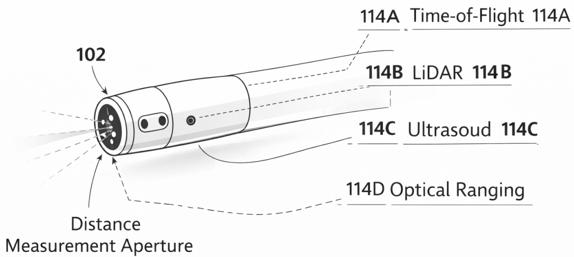
FIG. 4B Example Distal Sensing Tip
