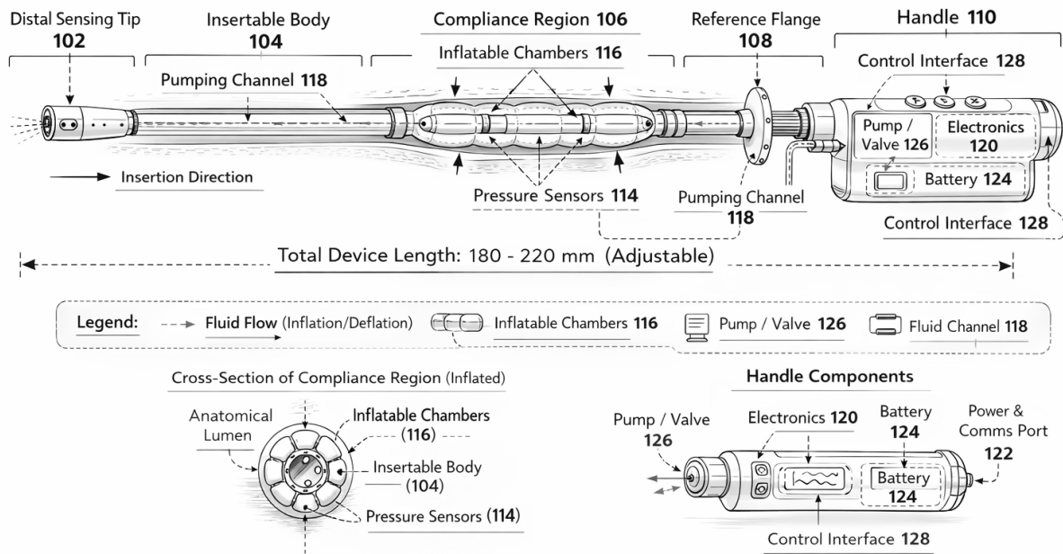
FIG. 4F Fluid Flow & Inflation System
