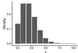
Poisson distribution
