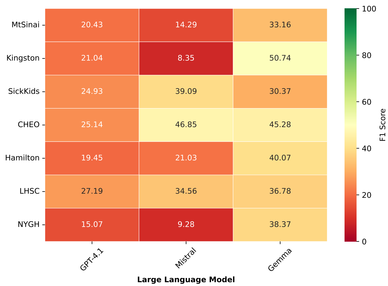
B) Vision-based LLM Performance
