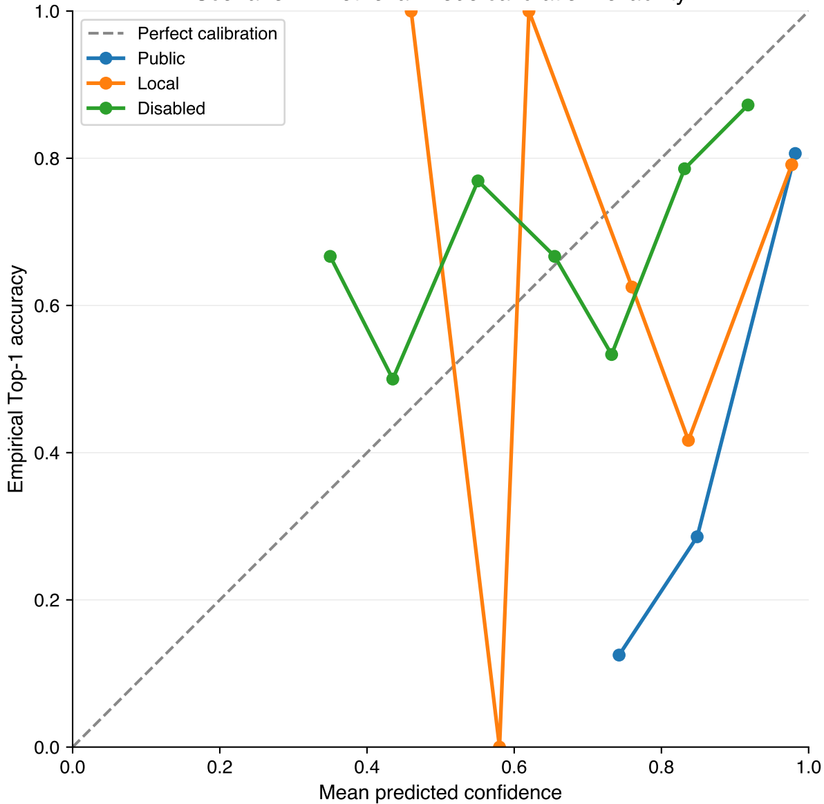
Scenario 2 -- retrieval-mode calibration reliability
