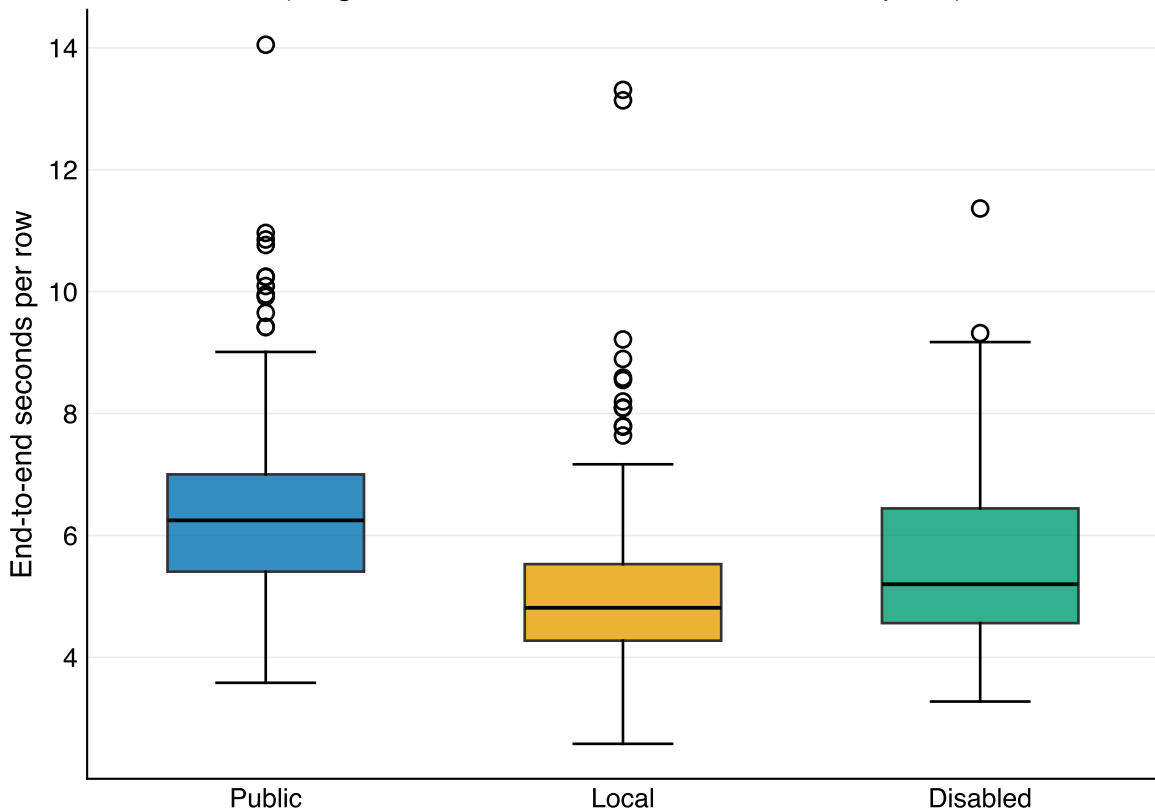
End-to-end latency by retrieval mode (n=218/mode) (stage-level breakdown omitted -- see caption)
