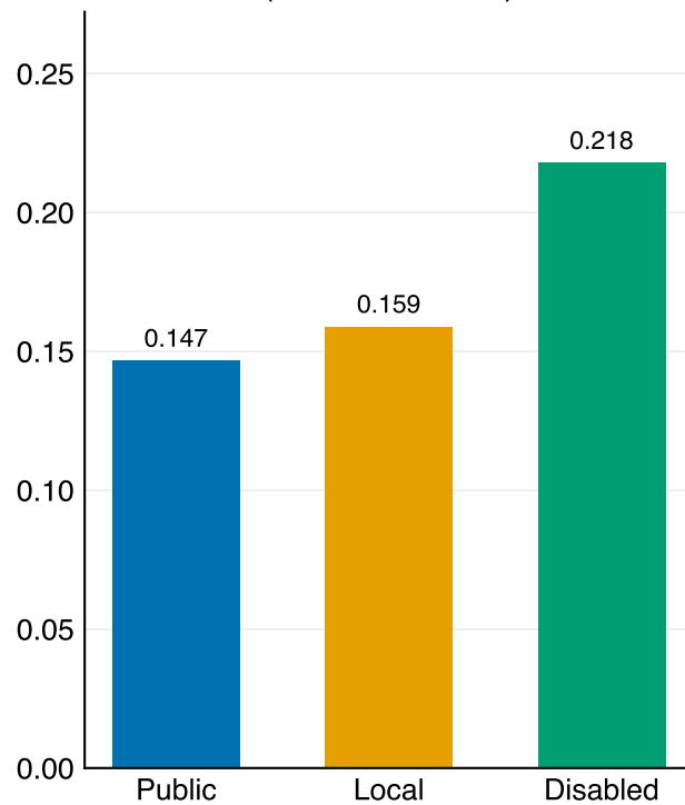
Brier score (lower is better)
