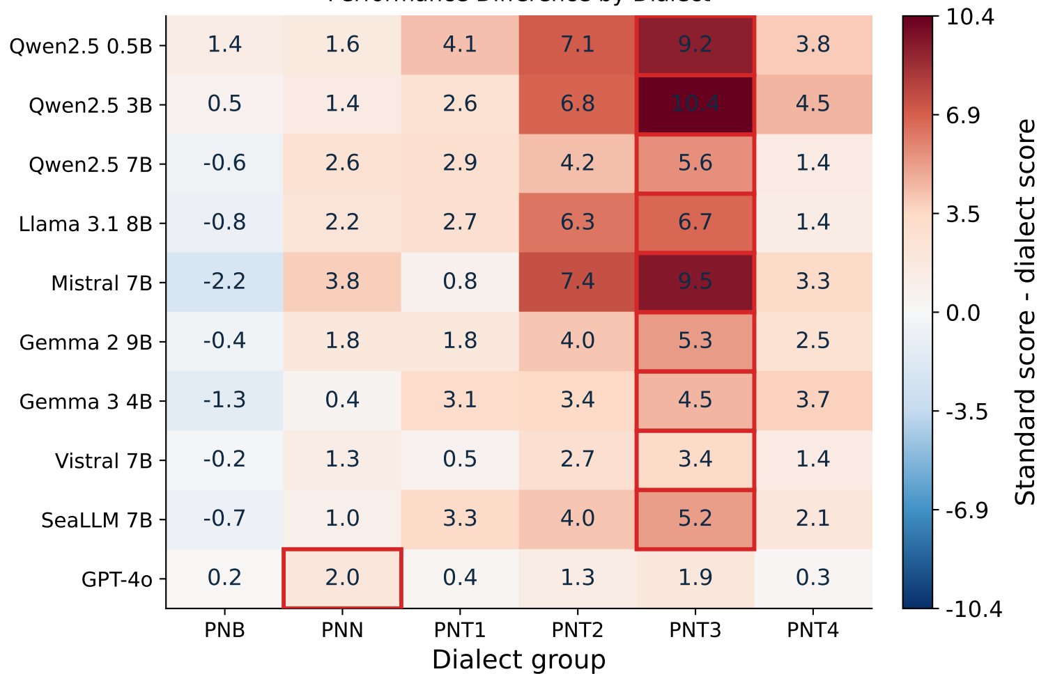
Performance Difference by Dialect
