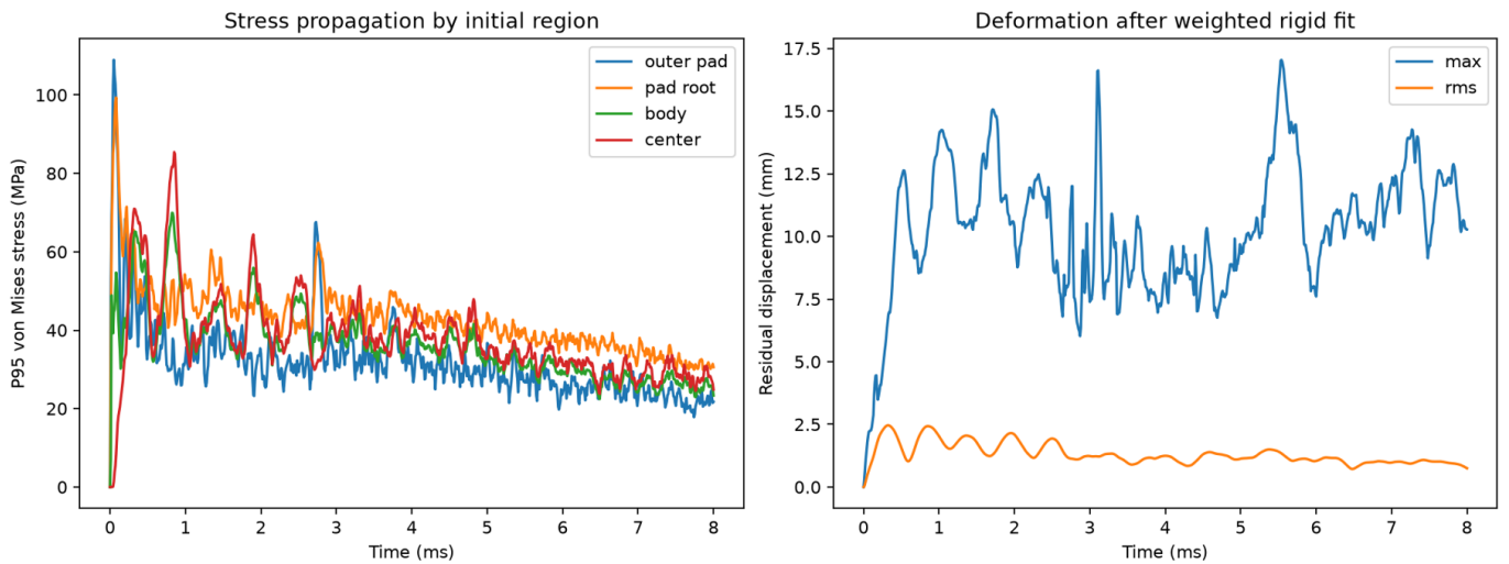
stress-propagation-deformation.png
