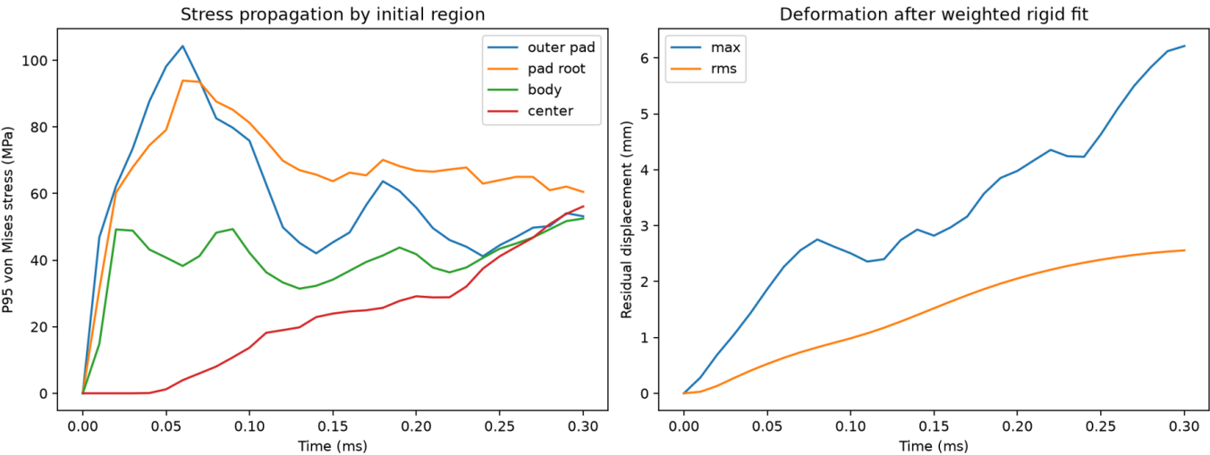
stress-propagation-deformation.png
