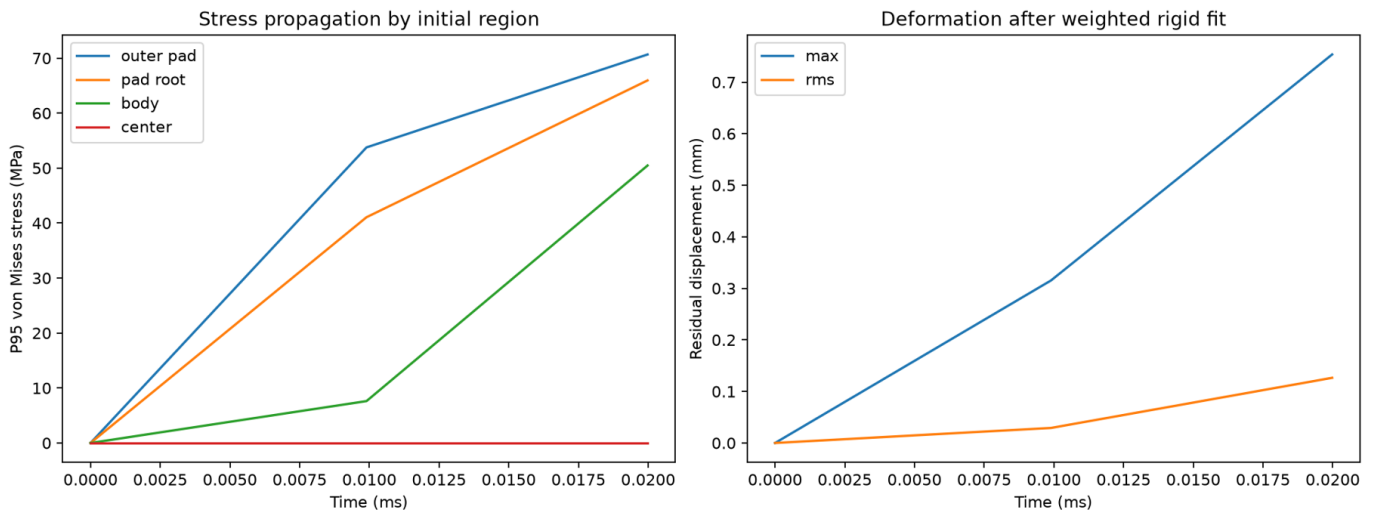
stress-propagation-deformation.png
