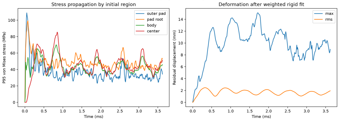
stress-propagation-deformation.png
