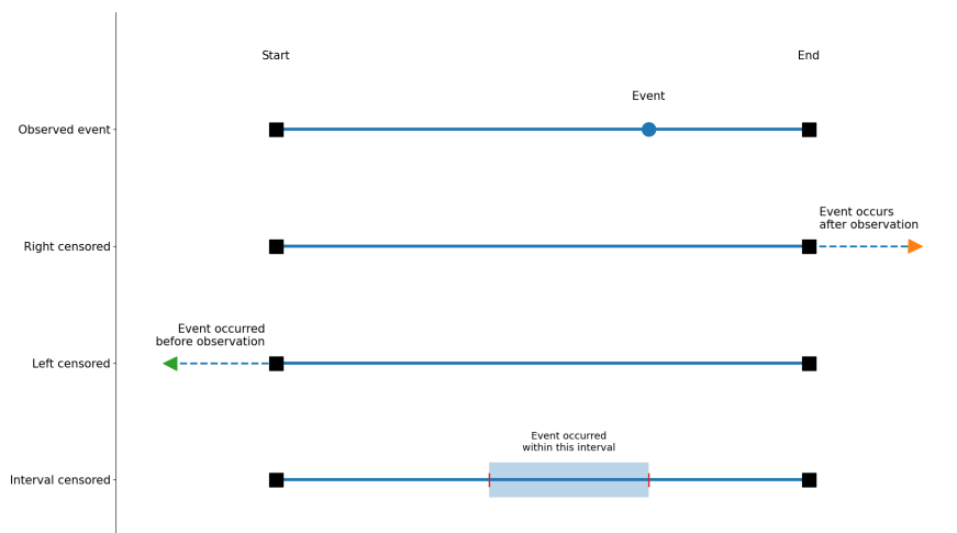
Figure 1 – Illustration of observed events and censoring types in survival analysis: observed event, right censoring, left censoring, and interval censoring.
