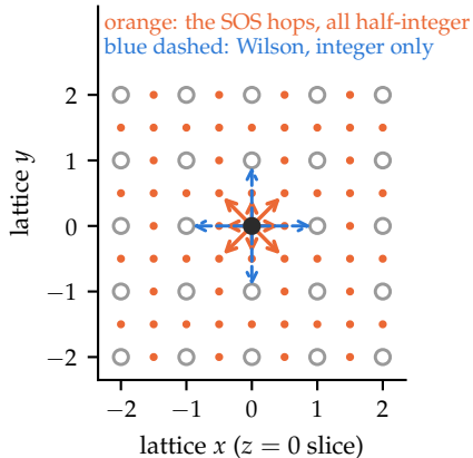
(b) the reason: the flux's squares sit on the half-offset lattice
