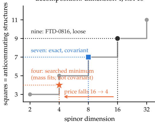
(d) the price is set by the SHORTEST decomposition: dimension 4, not 16
