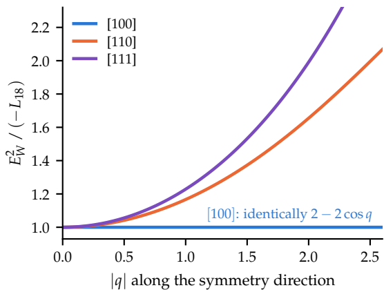
(a) exact along the axes, wrong off them: the mismatch is angular
