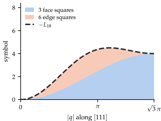
(c) one decomposition, not the fewest: nine squares stack onto the symbol
