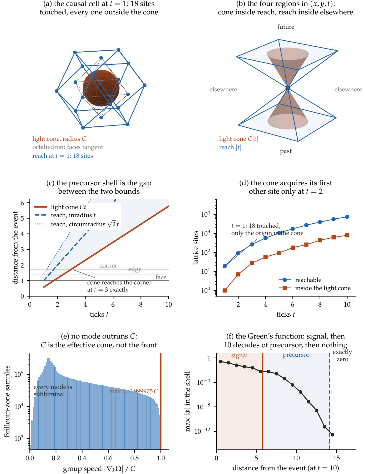
Figure 20: The complete causal partition around one event. (a) At t = 1 the light-cone sphere is inscribed in the octahedron — its inradius is C , so the eight faces are tangent — which is itself inside the reach polytope. (b) Past, future, and elsewhere in (x, y, t) , with the round cone strictly inside the square-sectioned reach. (c) The precursor shell is the gap between the two bounds; the cone closes over the body diagonal at t = 3 exactly. (d) At t = 1 eighteen sites have been touched and only the origin lies in the cone. (e) Every finite-wavelength mode is strictly subluminal, so no propagating mode outruns C — making it the effective cone, not the strict front, which is the reach boundary. (f) Across the shell the Green's function falls ten decades and then terminates in an exact zero.
