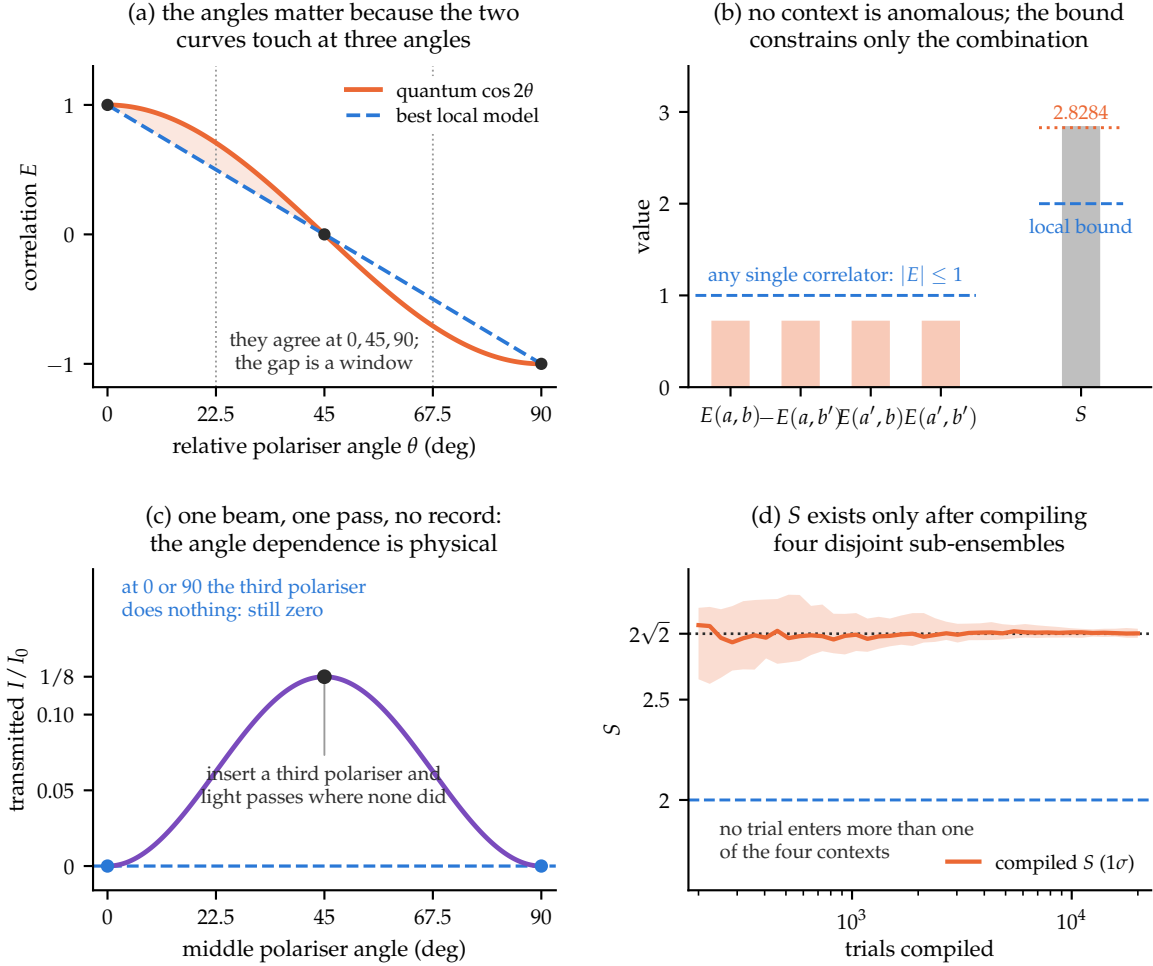
Figure 10: The angles, and the boundary. (a) For polarisation-entangled light the quantum correlation \cos 2\theta and the best local model — a straight line — touch at 0^\circ , 45^\circ and 90^\circ , so the violation is an angle window rather than a uniform excess; the widest single gap is 0.211 at 19.85^\circ . (b) At the CHSH settings each of the four contexts contributes exactly 1/\sqrt{2} , well inside the |E| \leq 1 available to any correlator: no context is individually anomalous, and the local bound constrains only the total. (c) Two crossed polarisers transmit nothing; inserting a third at 45^\circ transmits I_0/8 . One beam, one pass, no ensemble comparison and no record — the angle dependence is physical, not a feature of the bookkeeping. (d) S by contrast is a compiled statistic: the four sub-ensembles are verified disjoint and exhaustive, no trial enters more than one, and the number exists only after all four are combined.
