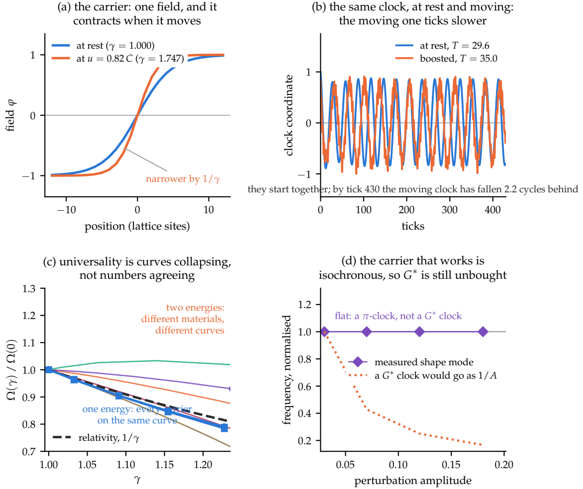
Figure 12: The carrier arc, watched rather than tabulated. (a) The carrier itself: one field, whose profile contracts by 1/\gamma when it moves. (b) The claim, directly. The internal clock's trace at rest and boosted, released in phase: the moving clock has fallen 2.2 cycles behind by tick 430. The roughness on the boosted trace is real — a boosted lattice kink radiates. (c) Universality as convergence. Two-category carriers fan apart, one of them running faster when moving; measured as a spread in the frequency ratio \Omega/\Omega_0 at \gamma = 1.22 , they span 0.283 against the one-energy carriers' 0.006, a factor of 46. (The body quotes the same comparison as a spread in the fitted exponent , 1.76 against 0.043; the two pairs measure different things and neither is a restatement of the other.) The one-energy curves collapse onto each other and lie a little below 1/\gamma , the residual discussed in the text. (d) Why this is still not the G^* clock: the shape-mode frequency is flat in amplitude — isochronous to \leq 0.23\% , set by the FFT bin — where a quartic clock would fall as 1/A .
