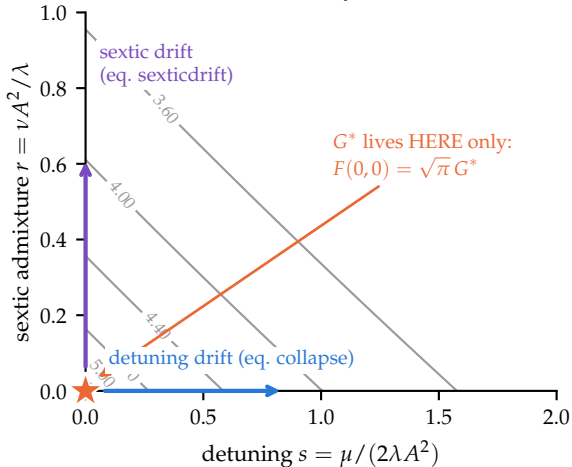
(b) the double limit: two independent drifts, and the constant only at their corner
