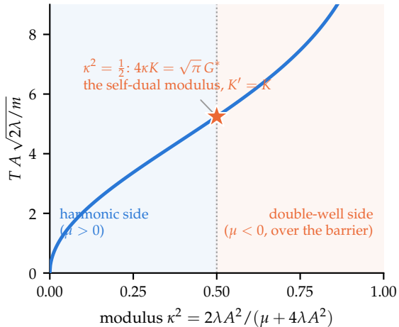
(a) one curve carries every detuning: the universal collapse 4\kappa K(\kappa)
