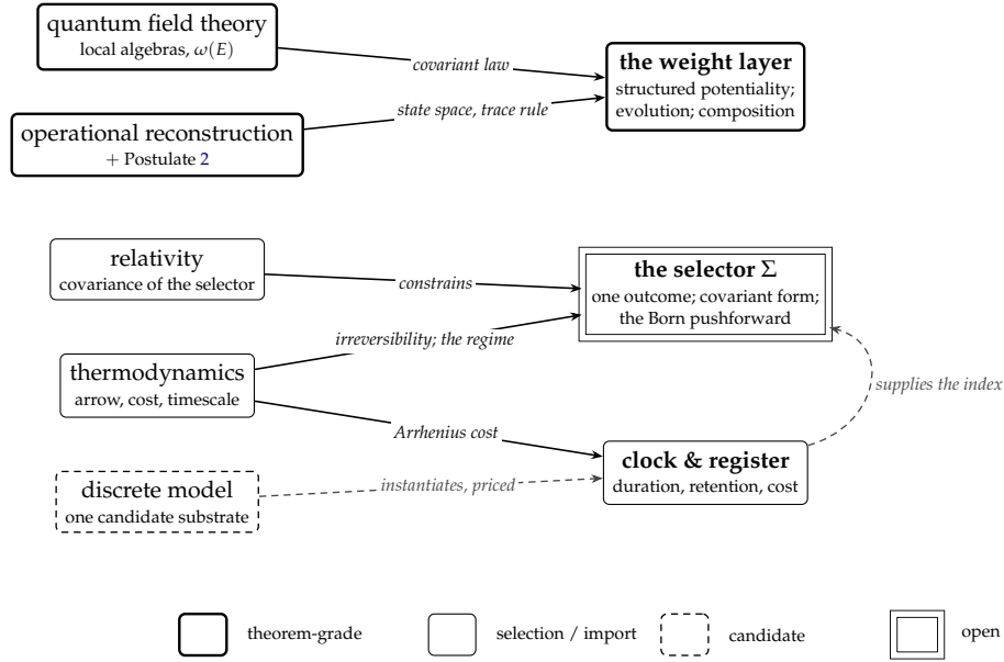
Figure 21: What supplies what. Shapes encode status, never colour, as shown in the legend: solid for theorem-grade within stated premises, thin for selections and imported representations, dashed for a candidate instantiation, double-ruled for the paper’s one open object. Solid arrows are constructions; the dashed arrow marks a candidate instantiation that is priced rather than free. The weight layer is supplied twice over and is the settled part of the architecture; the selector is supplied by no one, which is the paper’s point.
