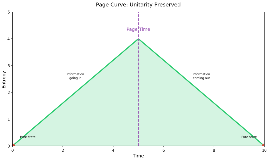
Figure 67.2: The Page curve showing entanglement entropy evolution during black hole evaporation.
