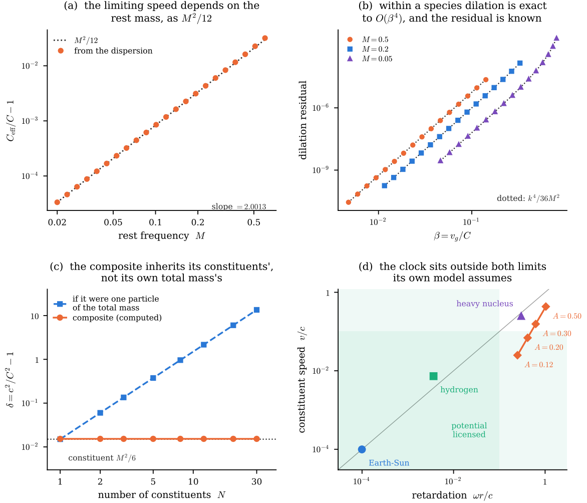
Figure 13: The cone arc of Sections 8.7–8.9, computed. (a) The limiting speed extracted from the exact dispersion tracks M^2/12 ; the fitted log–log slope is 2.0013. (b) Using each species’ own C_{\text{eff}} , the dilation relation fails only at O(\beta^4) , and the residual follows the analytic k^4/36M^2 (dotted) to within 1.1% across three masses. (c) The composite result: a bound object’s excess is its constituents’, constant to seven digits as the constituent number runs 1 \rightarrow 30 , while the reading that treats it as one particle of the total mass grows as N^2 . (d) The two limits hidden in a distance potential, with real systems placed. Orbits lie on the diagonal because \omega r = v for them; the mechanical clock does not, and sits outside the licensed corner on both axes — more relativistic internally than a heavy nucleus.
