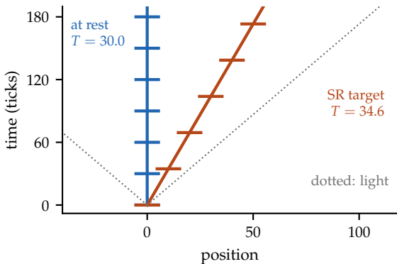
(e) special-relativistic target (schematic): moving ticks are further apart
