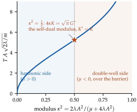
(a) one curve carries origin-crossing motion: the universal collapse 4\kappa K(\kappa)
