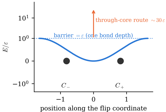
(a) the geometric bit: two states, barrier \varepsilon
