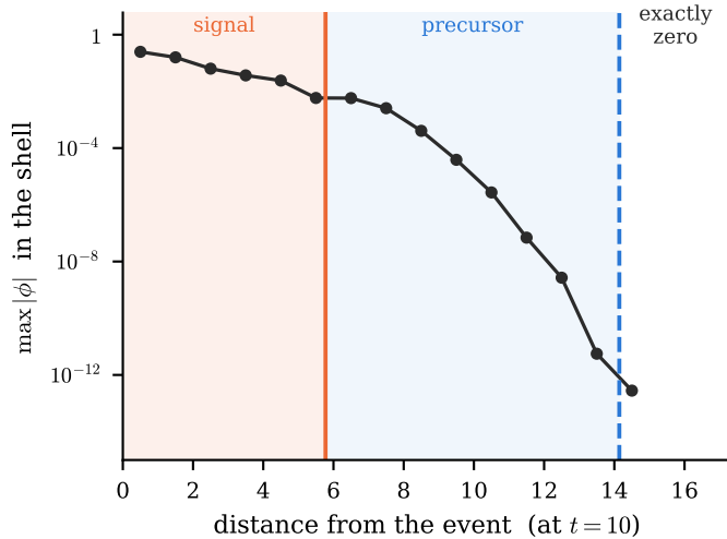
(f) the Green's function: signal, then 10 decades of precursor, then nothing
