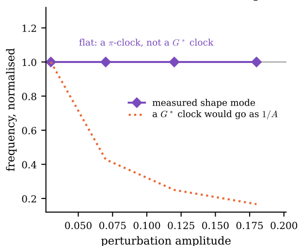
(d) the carrier that works is isochronous, so G^* is still unbought
