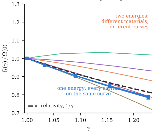
(c) universality is curves collapsing, not numbers agreeing
