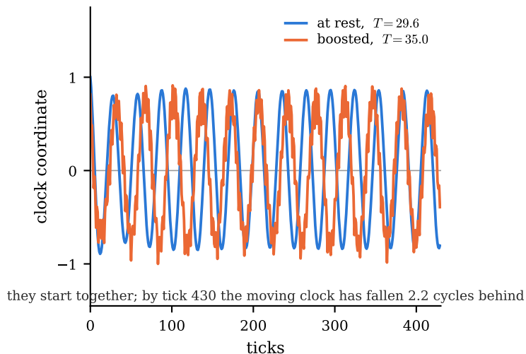
(b) the same clock, at rest and moving: the moving one ticks slower
