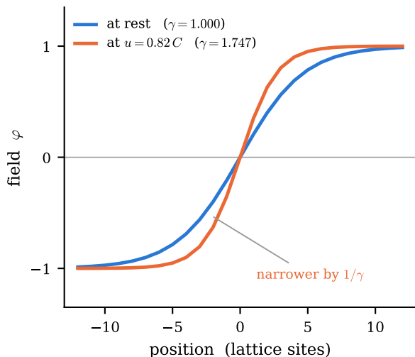
(a) the carrier: one field, and it contracts when it moves
