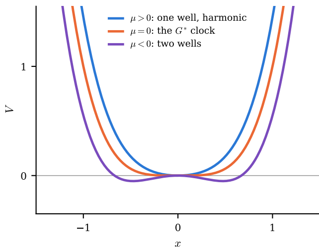
(c) the clock lives on one surface: the threshold between one well and two
