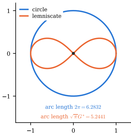
(a) the constants are the curves: \pi for one, G^* for the other
