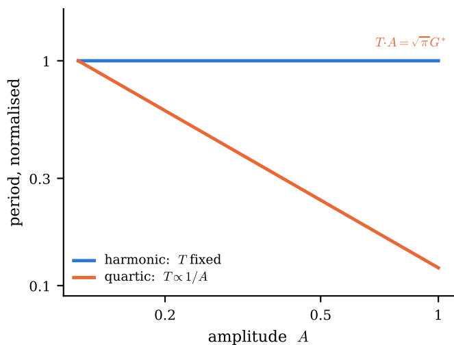
(f) and the behaviour that follows: one ignores amplitude, one counts it
