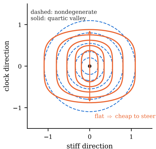
(d) degeneracy, seen: the valley opens along the clock direction
