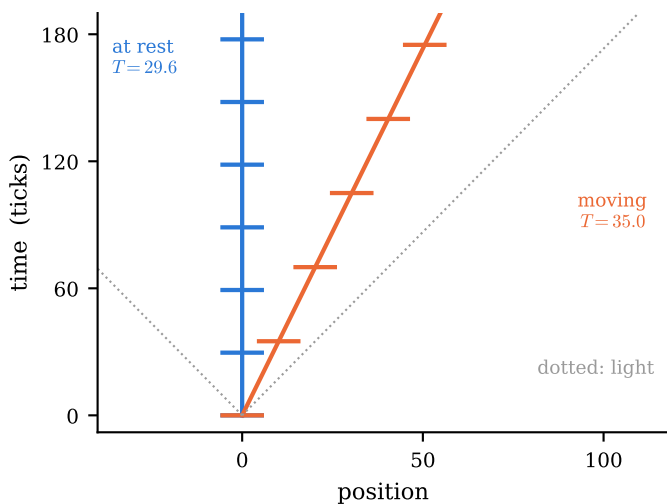
(e) dilation, seen: the moving clock's ticks are further apart in time
