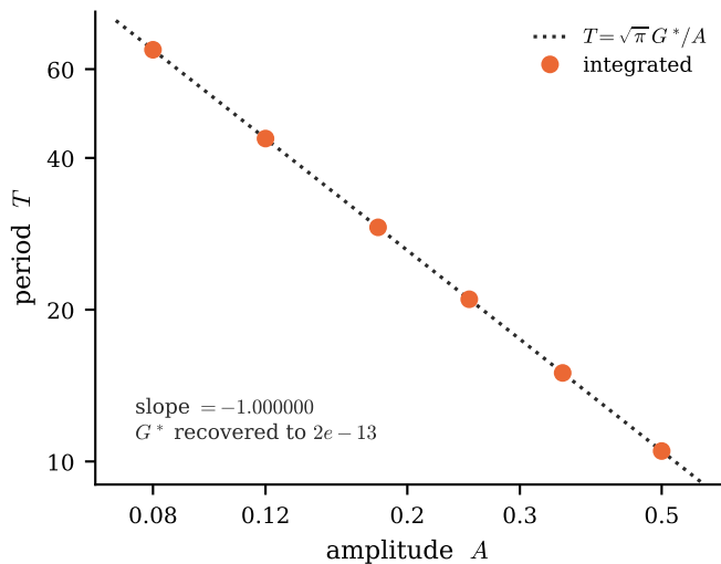
(c) the clock law, with no fitted scale: slope -1 and the constant is G^*
