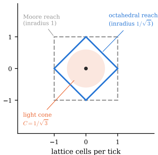
(a) substrate: the light cone sits inside every candidate causal polytope
