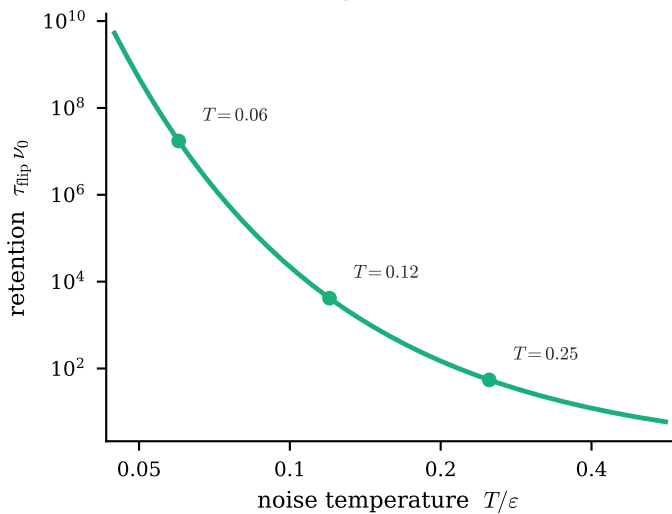
(e) retention is Arrhenius:
