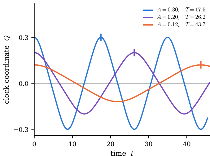
(b) clock: a bigger swing is a faster clock (ticks mark one period)
