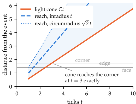
(c) the precursor shell is the gap between the two bounds
