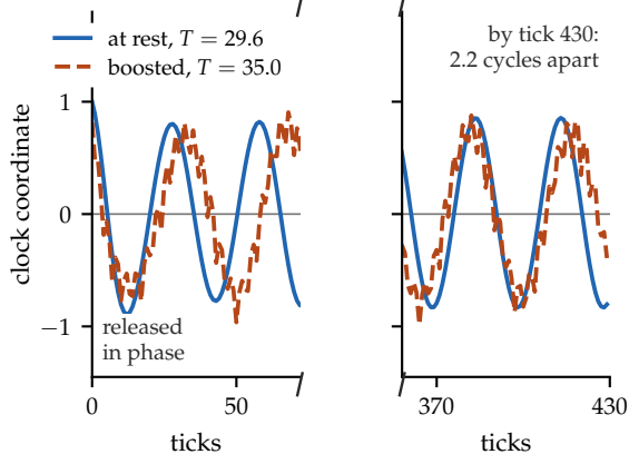
(b) the same clock, at rest and moving: the moving one ticks slower
