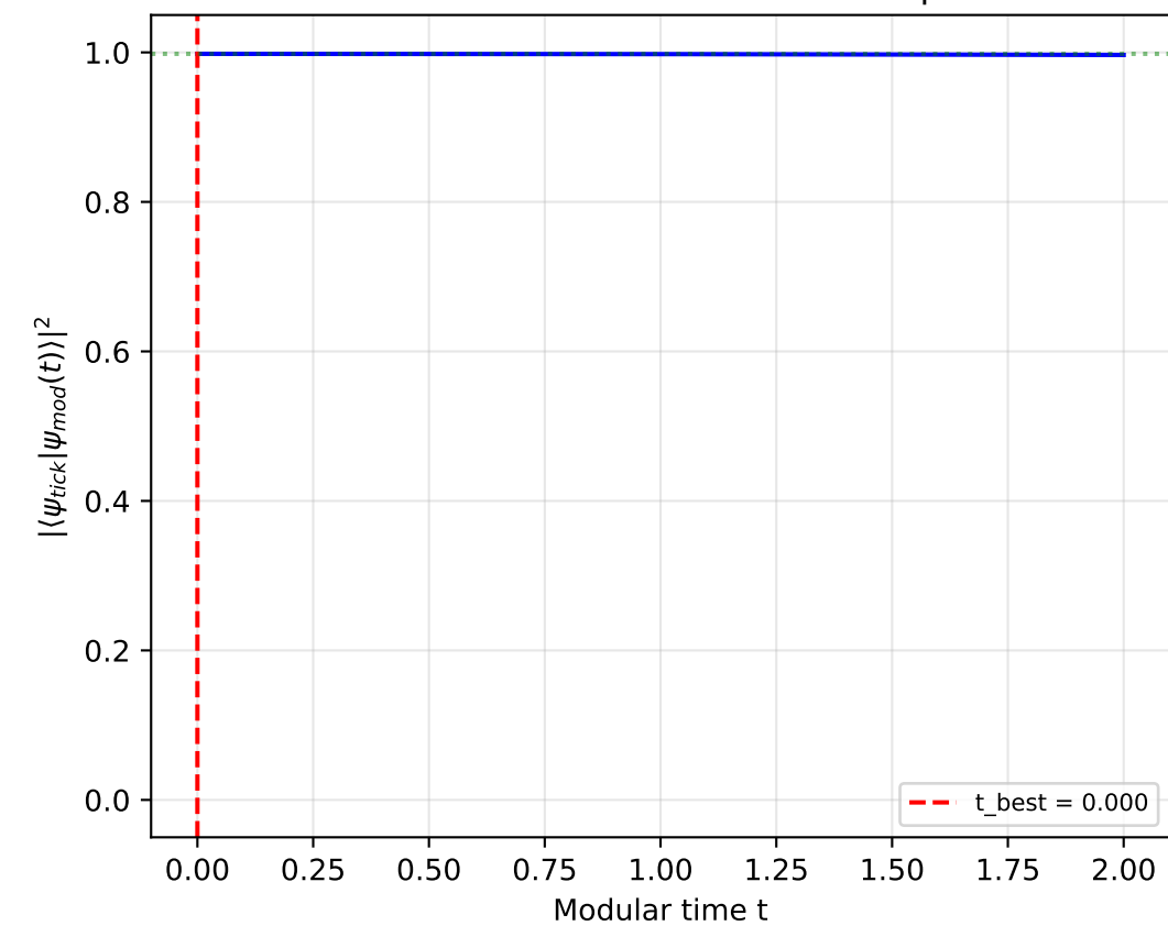
C: Tick vs Modular Flow Overlap
