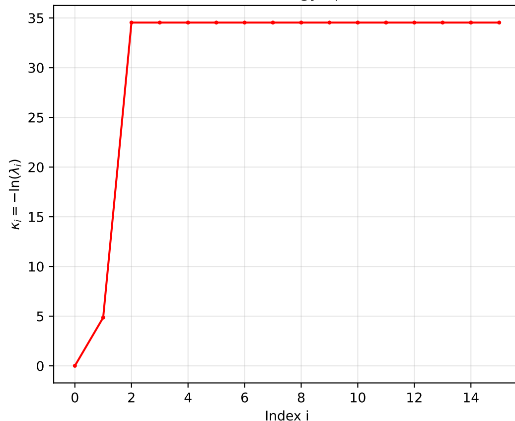
D: Modular Flow vs Tick Evolution
