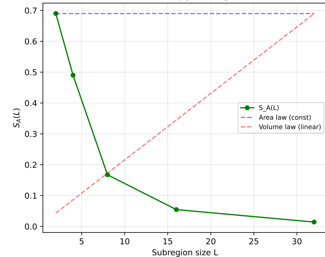
C: Entropy Scaling
