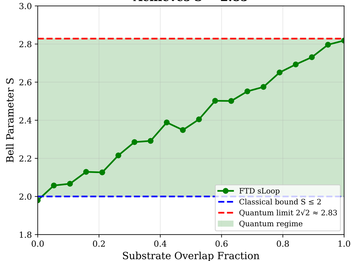
(C) Bell Violation via sLoop
