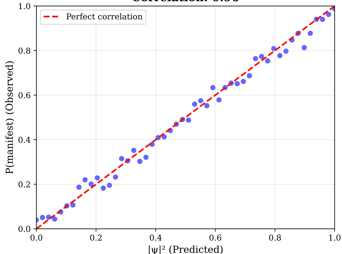
(B) Born Rule Emergence
