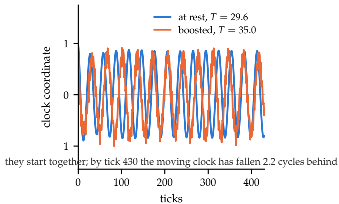
(b) the same clock, at rest and moving: the moving one ticks slower
