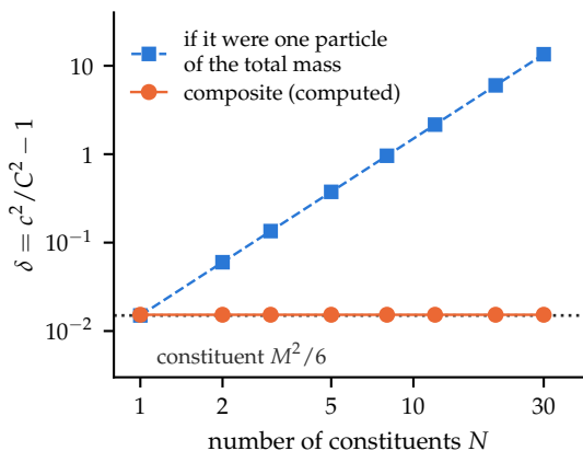
(c) the composite inherits its constituents', not its own total mass's
