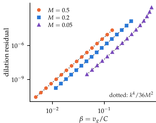
(b) within a species dilation is exact to O(\beta^4) , and the residual is known
