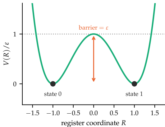
(d) register: two states, one barrier, and it is the same \varepsilon
