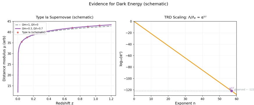
Figure 65.1: Evidence for dark energy from Type Ia supernovae: distant supernovae are fainter than expected in a decelerating universe, indicating accelerating expansion.
