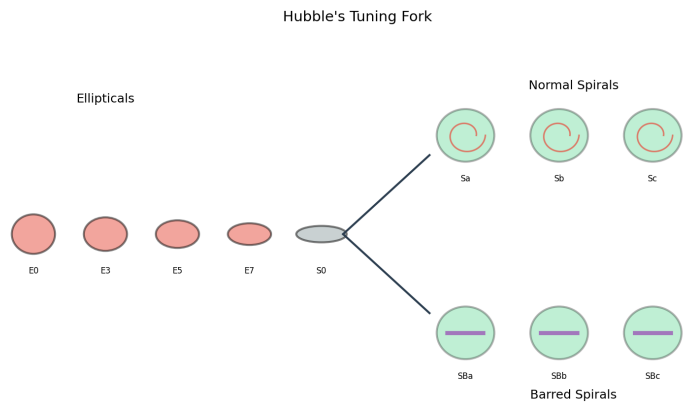
Figure 60.1: The Hubble tuning fork classification: ellipticals on the left, lenticulars at the junction, and spirals branching into normal and barred types on the right.
