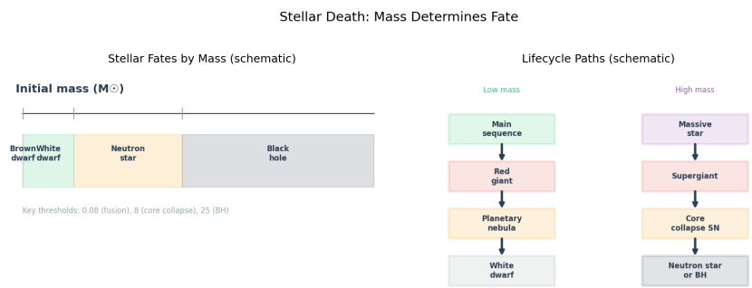
Figure 57.1: The pathways of stellar death: low-mass stars become white dwarfs via red giant and planetary nebula phases, while massive stars explode as supernovae leaving neutron stars or black holes.
