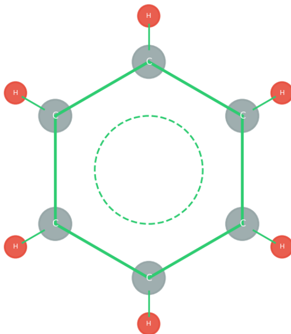
Benzene ( C_6H_6 ) - Aromatic ring with resonance
