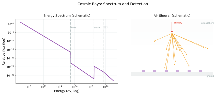
Figure 69.1: The cosmic ray energy spectrum showing three distinctive features: the “knee” at 3 \times 10^{15} eV where the spectrum steepens, the “ankle” at 3 \times 10^{18} eV where it flattens, and the GZK cutoff at 5 \times 10^{19} eV.
